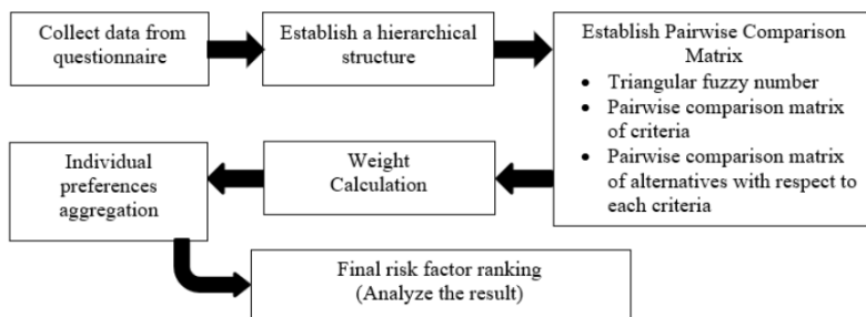
Figure 1: The Flowchart of FAHP Method
