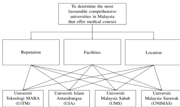
Figure 3: The Hierarchical Structure.
