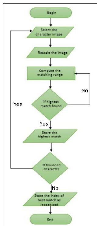
Figure 3 Template Matching Algorithm
