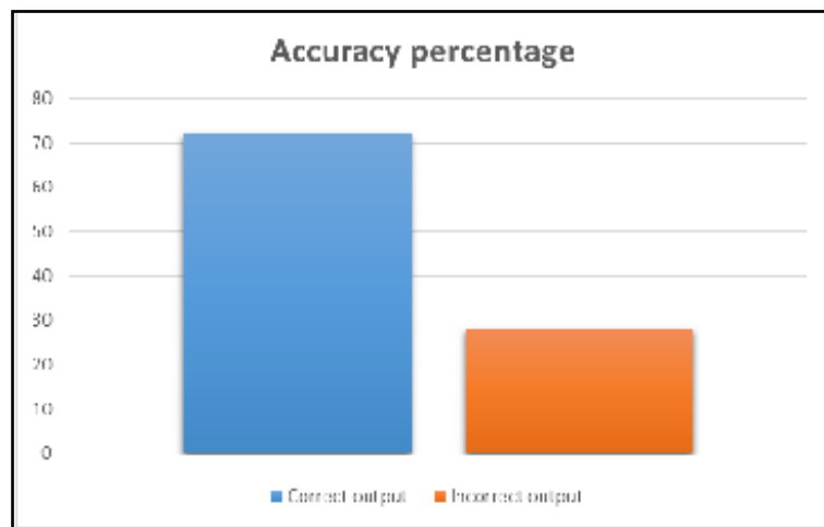
Figure 4 Accuracy Percentage
