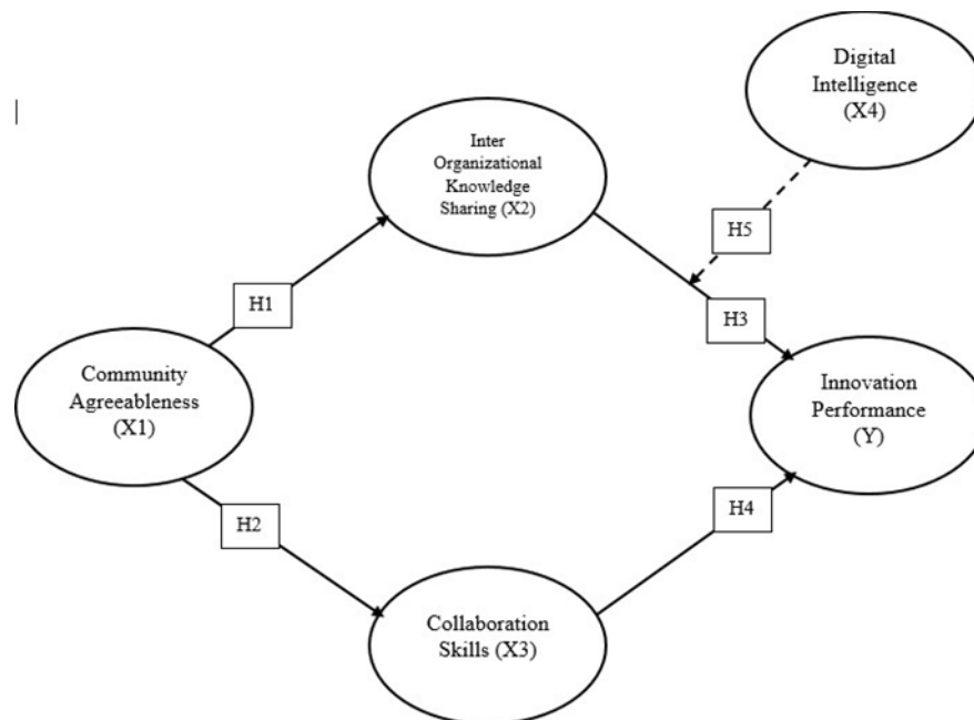
Figure 1. Research Framework
