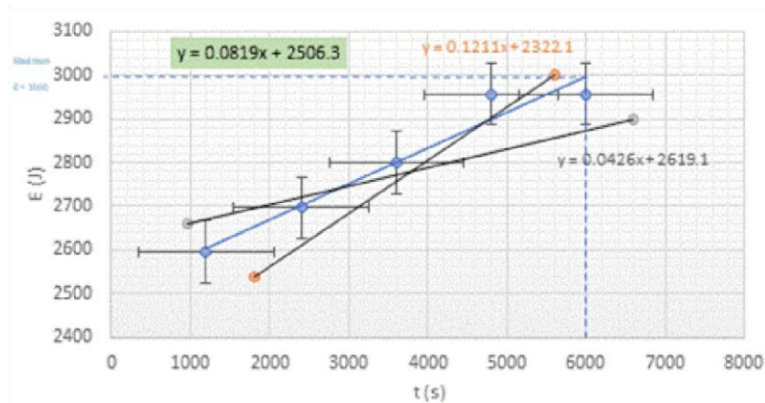
Graph 7: Electrical Energy (J) vs Time (s) for the series circuit
