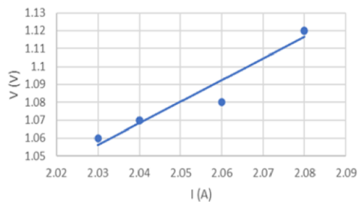
Graph 6: Voltage (V) vs Current (A) for the parallel circuit
