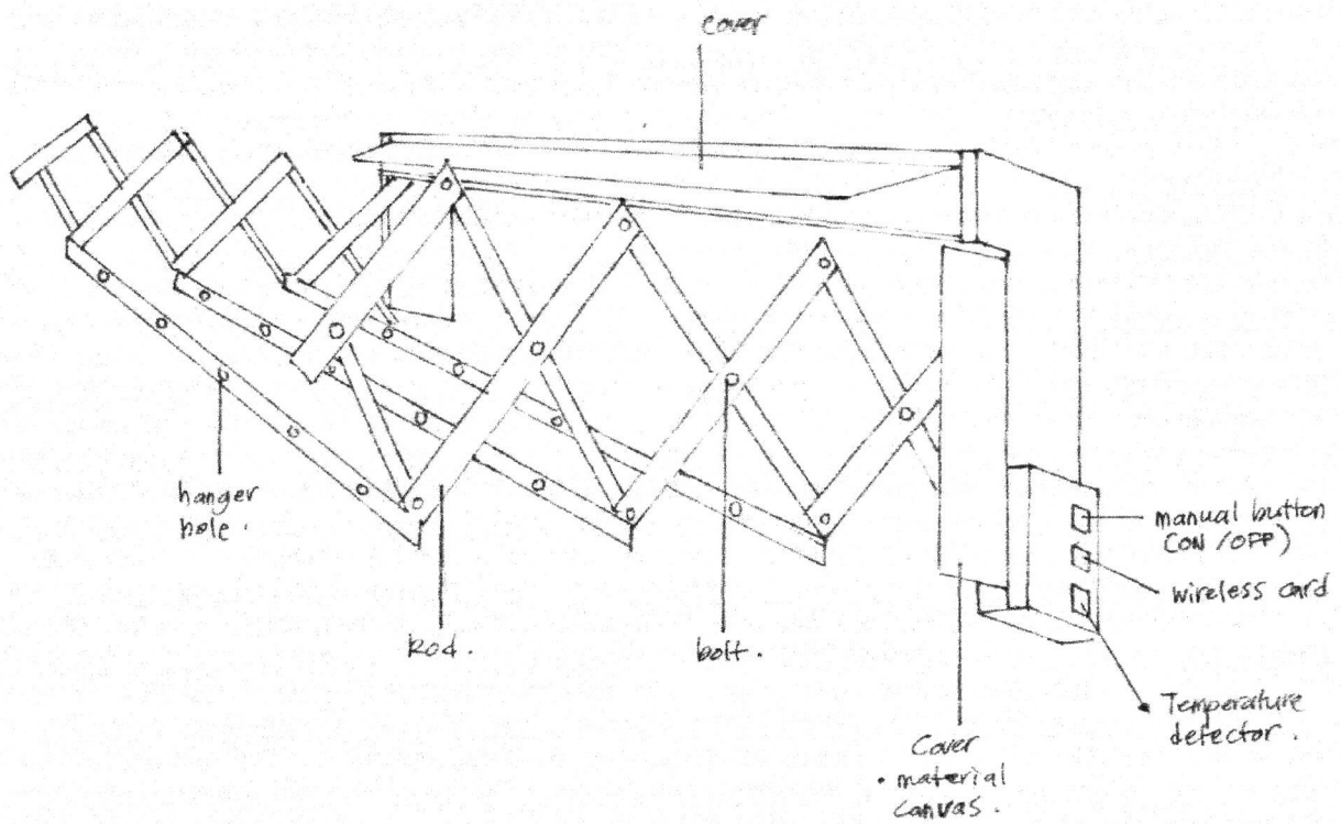
Figure 1: Component Part of Smart Drying Rack
