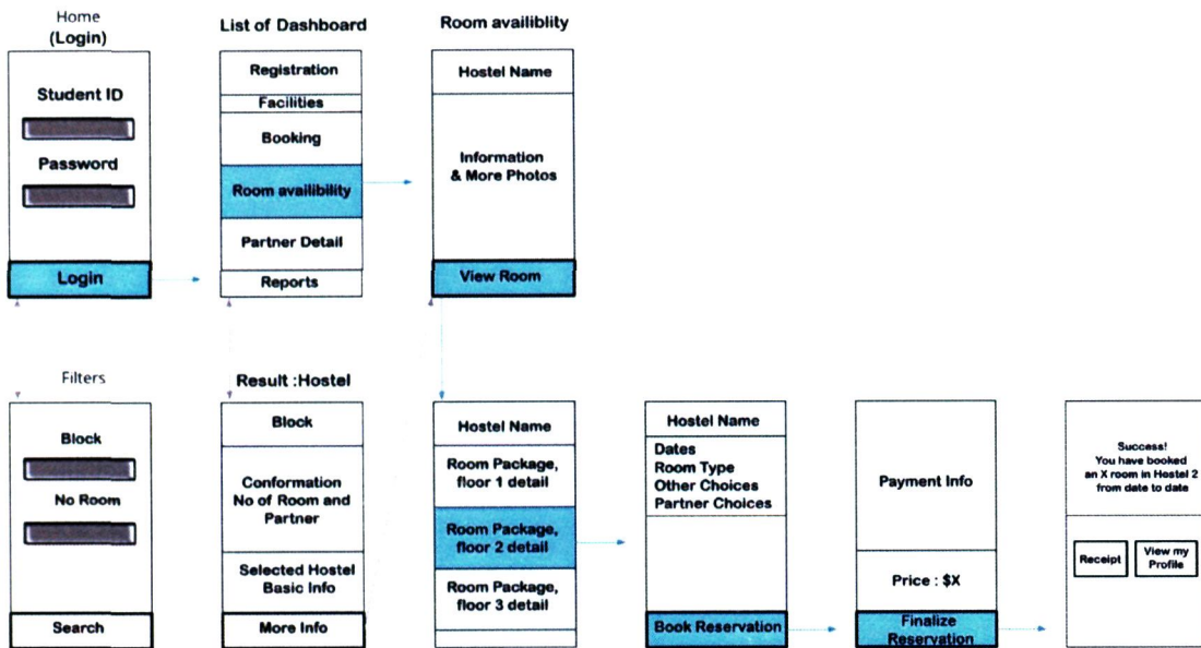
Figure 1.0: The Flow to Booking The Room and Choose the Partner
