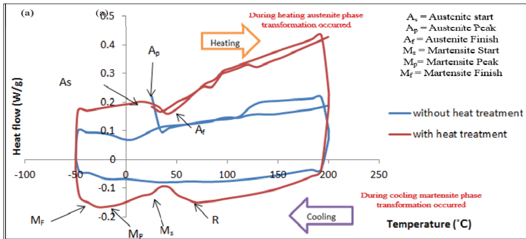
Figure 4 (a): DSC Curve for MIM with Composition of 50.0at% NiTi
