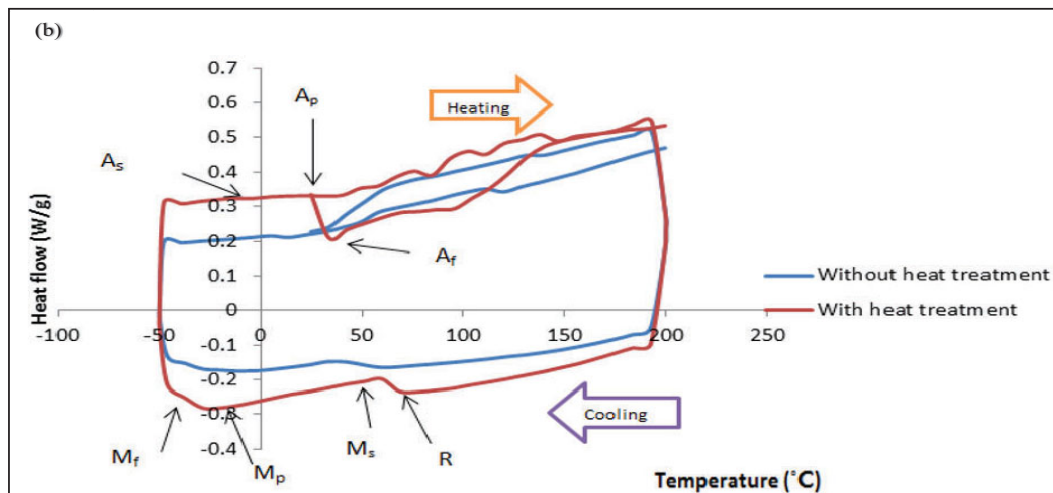
Figure 4 (b): DSC Curve for Composition of 50.8at% NiTi
