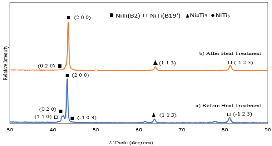
Figure 1(b): XRD Pattern of MIM 50.8at% NiTi
