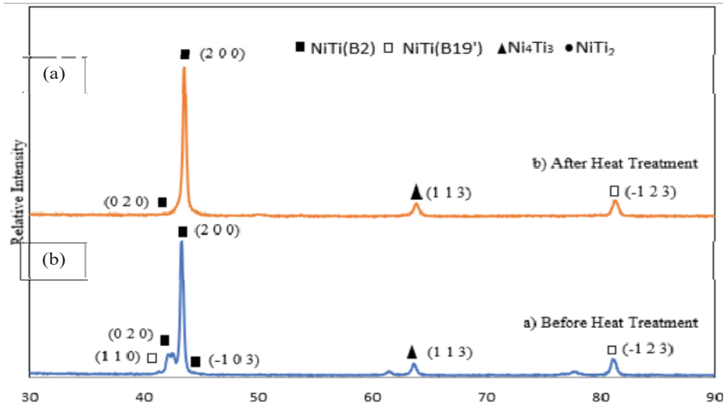
Figure 1(a): XRD Pattern of MIM 50.0at% NiTi
