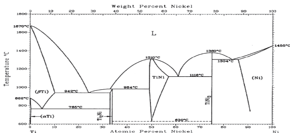
Figure 3: Binary Phase Diagram of NiTi Alloy [20]
