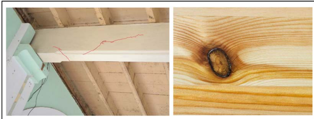
Figure 5 The beam number 18 has cracked due to timber knots. There are knots and crack that suspected can cause the beam to bend and will eventually break. Right: example of timber knots ( https://www.woodworkingnetwork.com/best-practices-guide , 2017)
