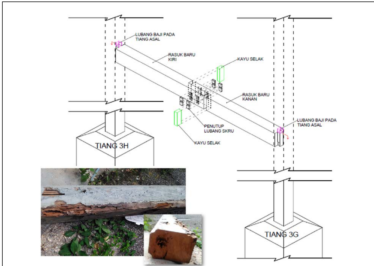
Figure 4 Diagram shows the new beam with proposed jointing in the middle in order to minimize the intervention on both pillars during restoration work. The left-below pictures show the decay of the original beam.
