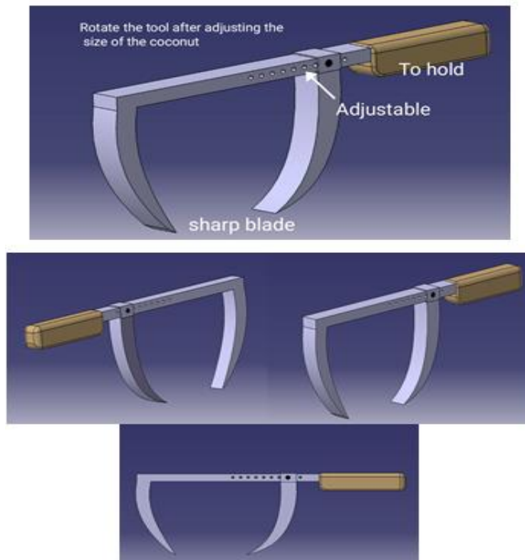
Figure 2.1: show the arrangement of the product (Cocopeeler)
