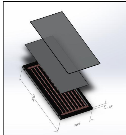
Figure 4: Flat-plate collector diagram
