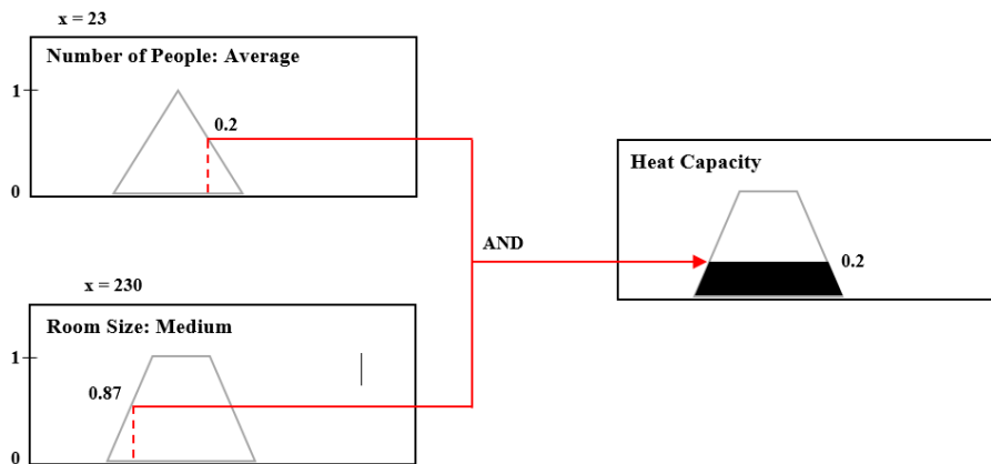
Figure 4: Rule Evaluation
