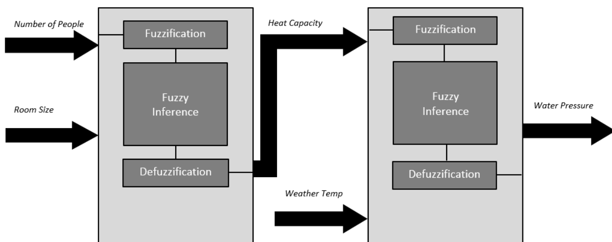
Figure 2: Fuzzy Logic Controller of Roof Sprinkler Cooling System
