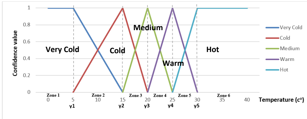
Figure 6: Membership function graph of weather temperature
