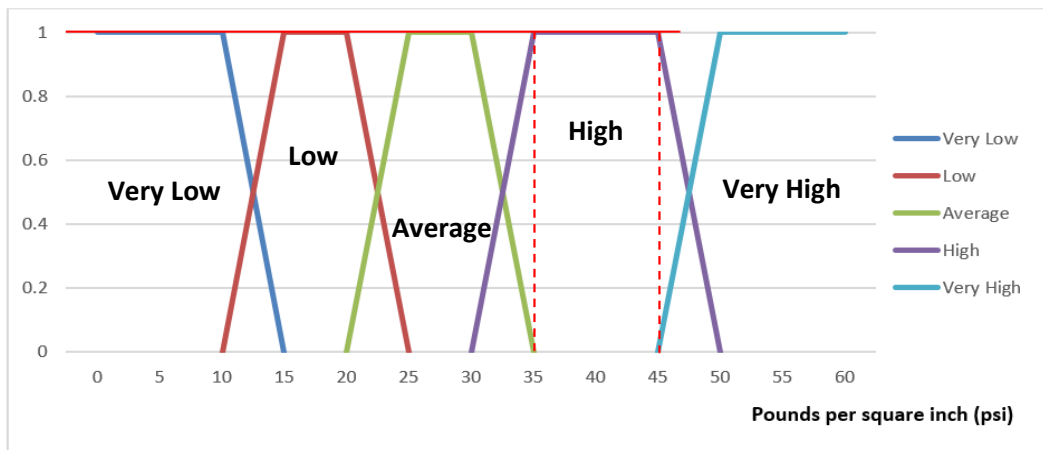
Figure 8: Membership function graph of water pressure
