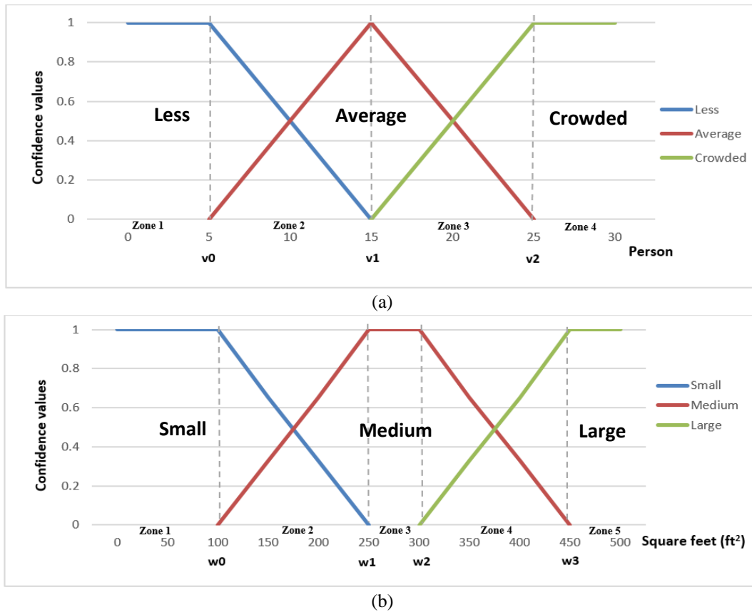
Figure 3: Membership function graph for (a) number of people and (b) room size
