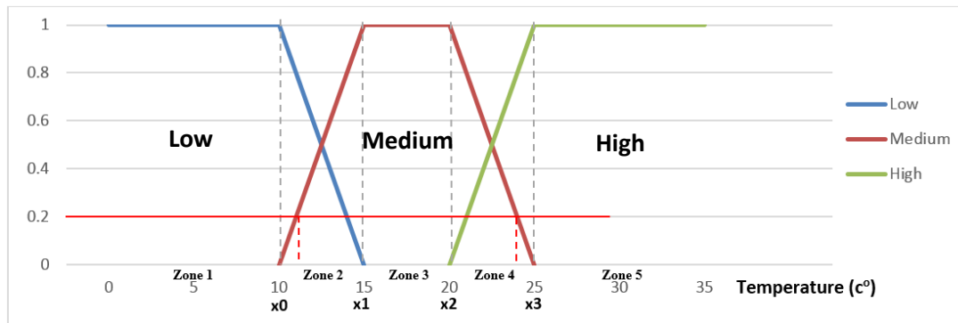
Figure 5: Membership function graph of heat capacity
