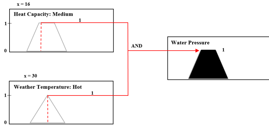
Figure 7: Rule evaluation for water pressure
