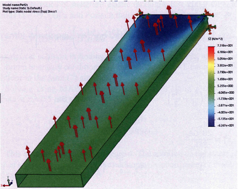
Figure 3b: Finite element analysis result
