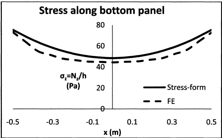
Figure 5: Stress distribution along bottom panel vs. distance x at clamping area
