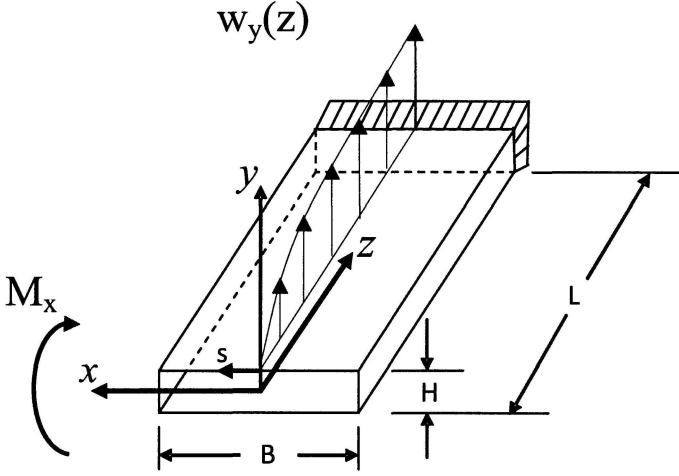
Figure 2: Box beam under transversal distributed load
