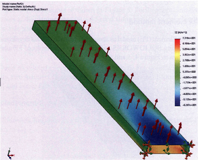
Figure 3c: Finite element analysis result
