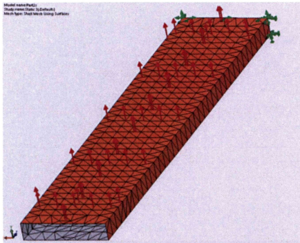
Figure 3a: Finite element model
