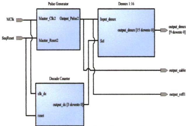
Fig. 11. Connection between Pulse Generator, Demux 1:16 and Decade Counter.
