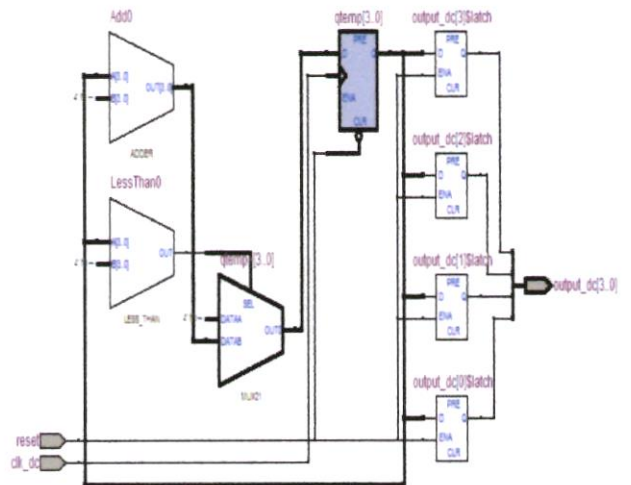
Fig. 10b. RTL for Decade Counter
