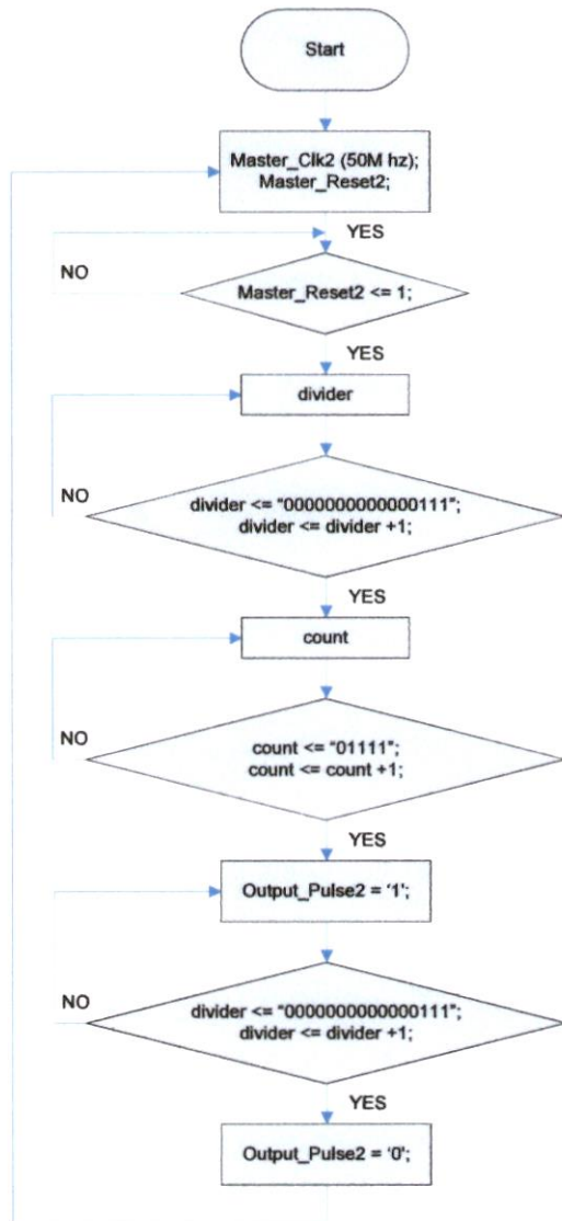
Fig. 5. Flowchart of Pulse Generator
