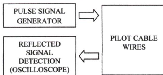
Fig. 1. Operation Block Diagram of TDR
