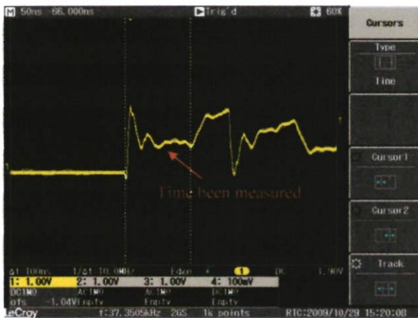
Fig. 17. TDR Measured Result and Pattern for Healthy Cable (100ns)
