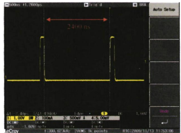
Fig. 16c. Result of 2400ns Delay between Pulses
