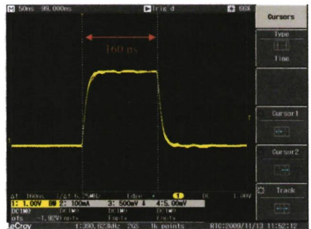
Fig. 16b. Result of 160ns Pulse Width
