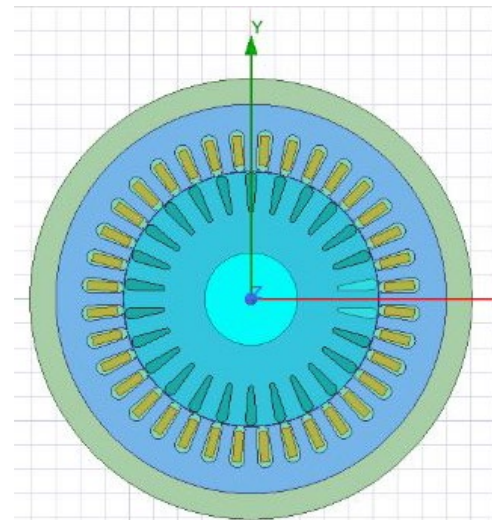
Fig. 3b. Induction Motor Model in Ansys Maxwell
