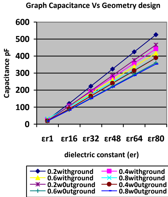
Figure 11. Graph Simulation Result
