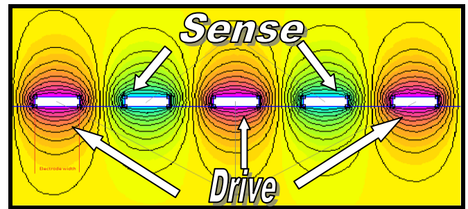
Figure 6. Simulation Result
