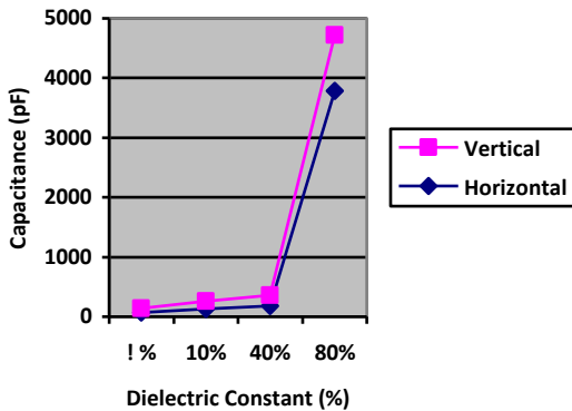
Figure 15. Graph Actual Hardware Testing
