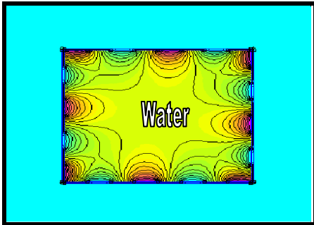
Figure 23. Square Box design Simulation with 10mm Electrodes width.
