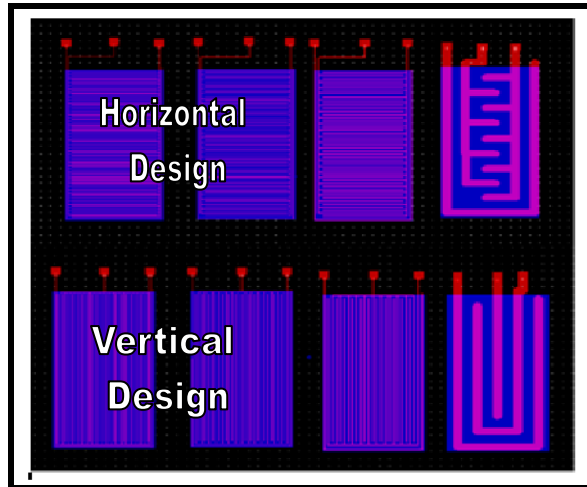
Figure 7. Design Plate Structure, Horizontal Electrodes (above) and Design Vertical Electrodes (below).
