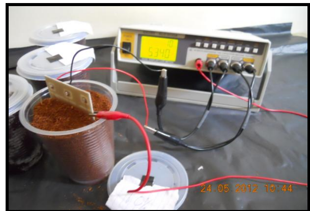
Figure 10. Test Set Up for FEF Soil Moisture Sensor
