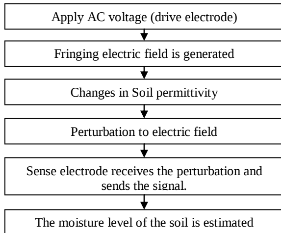
Figure 1. Principle of FEF Sensors [6]
