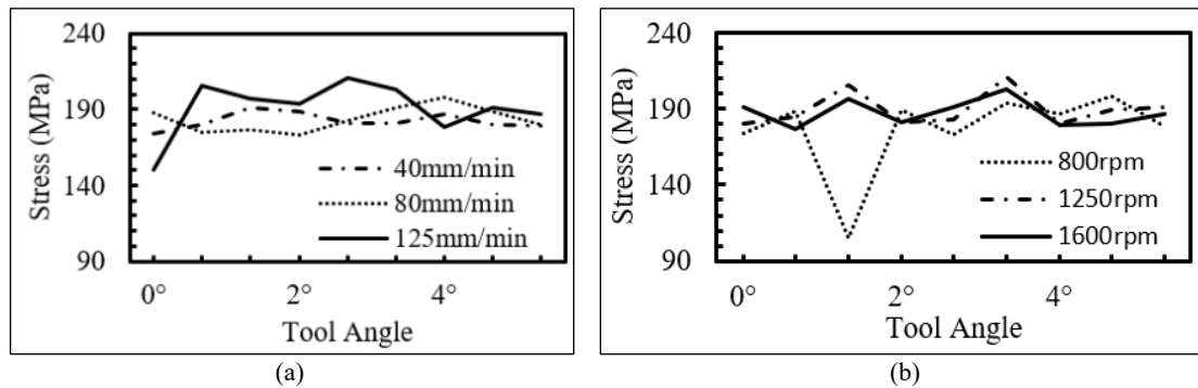
Fig. 9. Effect of tool angle on fracture stress at different (a) feed rate and (b) rotated-tool speed.
