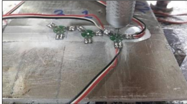
Fig. 6. Central drilling test (for residual stress test).
