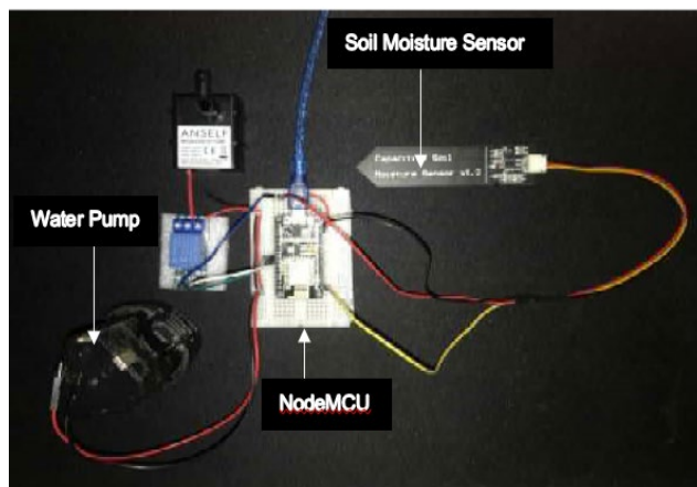
Fig. 6. Connection setup
