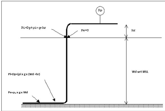
Figure 2 : Relationship between Design Pressure and Net Internal Pressure
