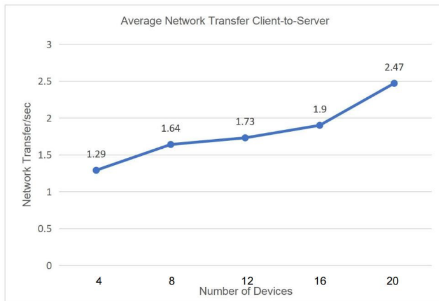
Fig. 3. Average network transfer Client to Server
