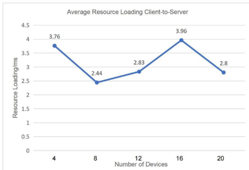
Fig. 5. Average Resource Loading Client to Server
