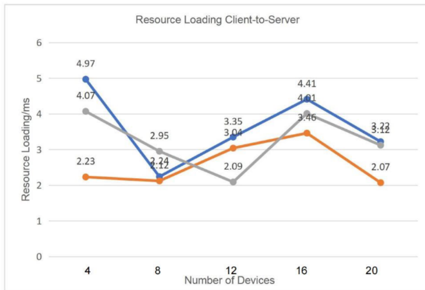
Fig. 4. Resource Loading Client to Server
