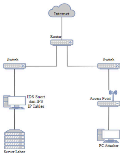
Fig. 3. Network architecture
