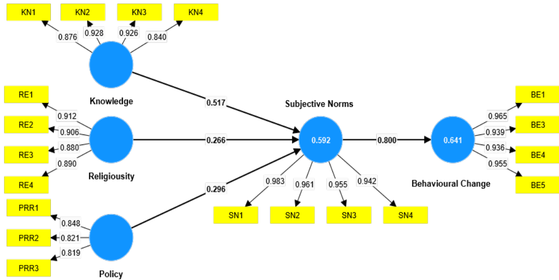
Figure 2. Measurement Model
