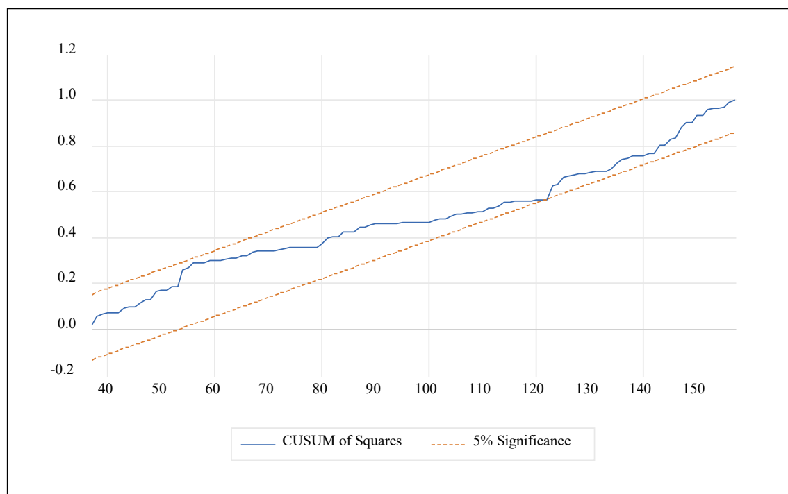
Fig. 2 CUSUMSQ Test for Market Performance (LNKLICI)
