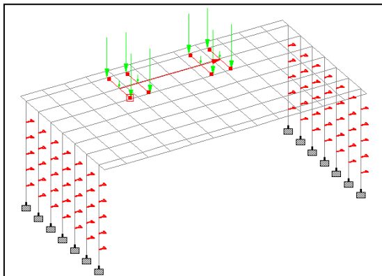
(c) H_B applied symmetrically in the bridge span
