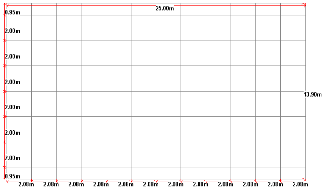
Figure 4: Grillage model of the single span bridge.
