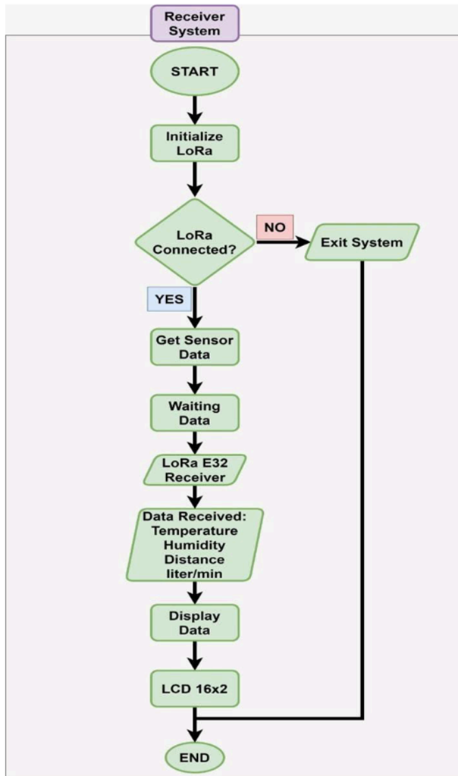
Fig. 3. Flowchart receiver
