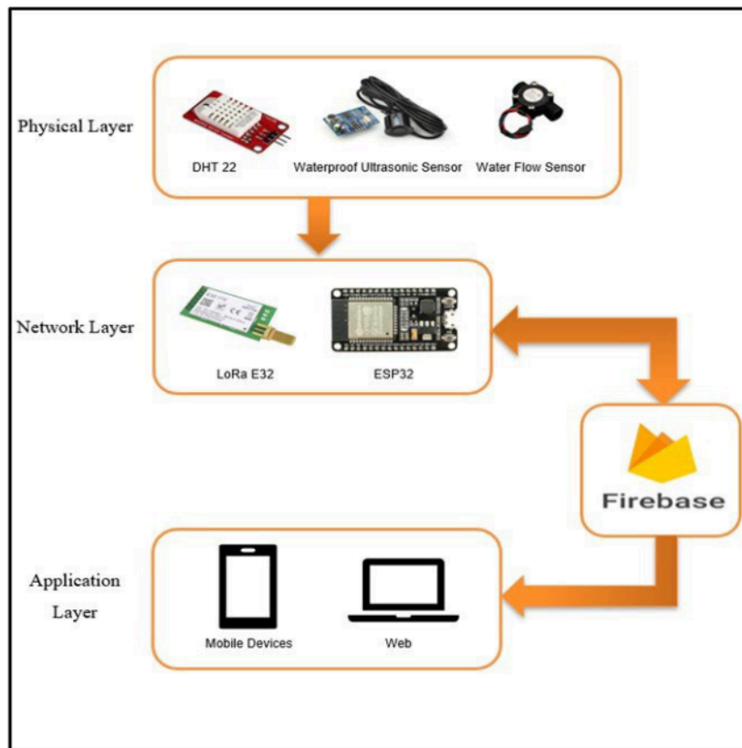
Fig. 4. System architecture
