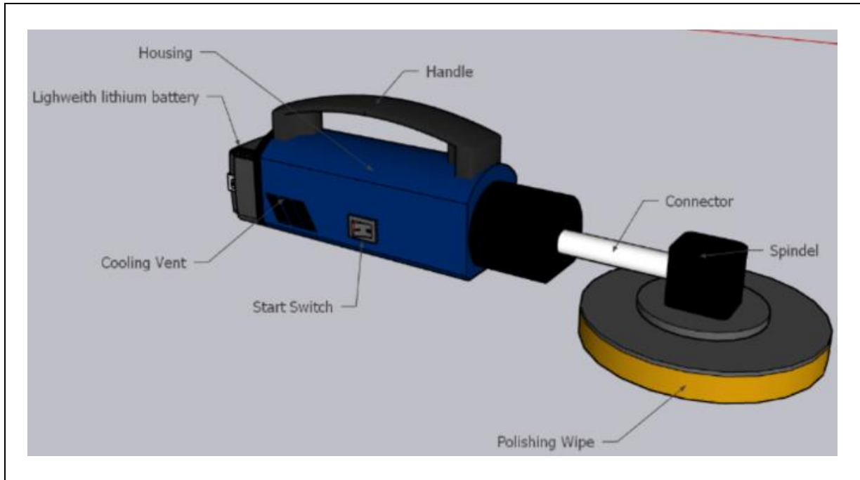
Portable Plaster Smoothing Machine
