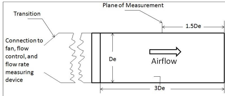
Figure 1 Schematic for minimum length for pipe installation
