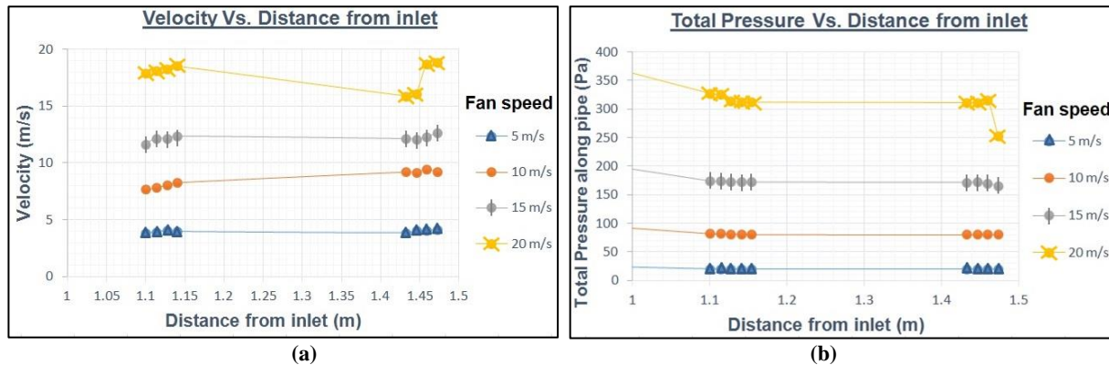
Figure 3 (a) Graph of velocity at the perforated holes, (b) Graph of total pressure distribution along the pipe
