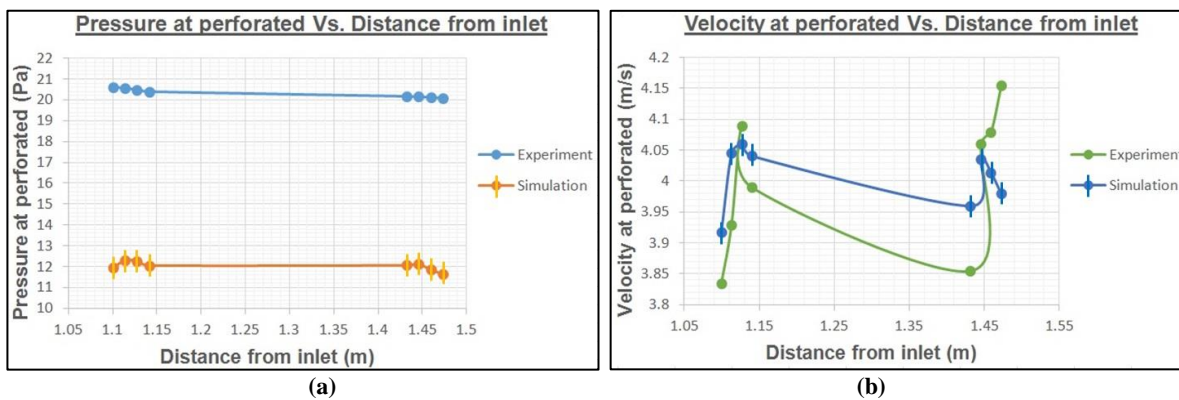
Figure 4 (a) Pressure distribution comparison between experimental and simulation at 5 m/s, (b) Velocity distribution comparison between experimental and simulation at 5 m/s
