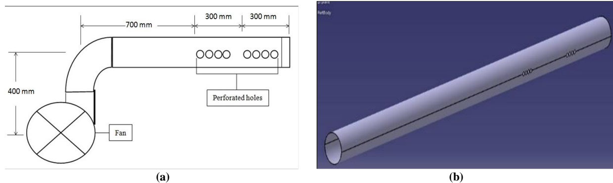
Figure 2(a) Schematic diagram for pipe installation for experiment, and (b) Model of Perforated Pipe for Simulation
