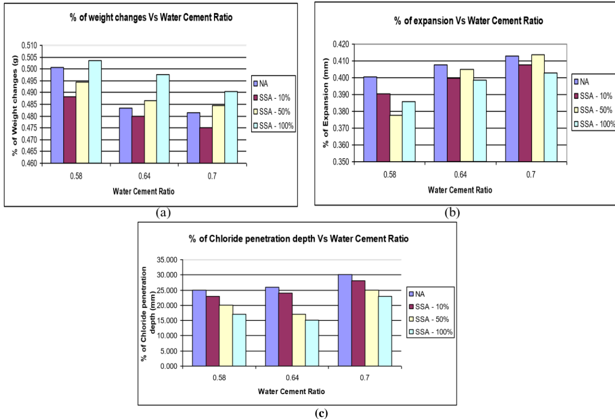
Figure 4 Concrete specimens made of various SS replacement level at various water cement ratio which is immersed 1M NaCl solution at 90 days. (a) Weight changes, (b) Expansion of dimension (c) Depth of chloride penetration
