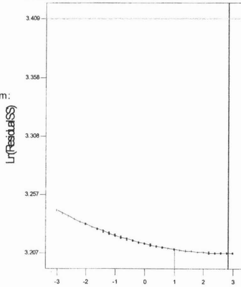
Box-Cox Plot for Power Transforms
