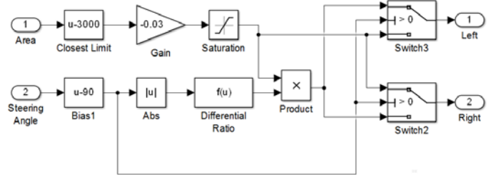
Fig. 7. SIMULINK model of the vehicle speed control algorithm
