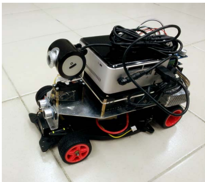
Fig. 1. System setup implemented on 1/18th scale car model
