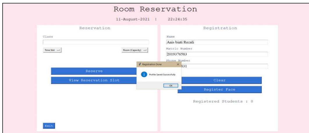
Figure 9: Profile saved
