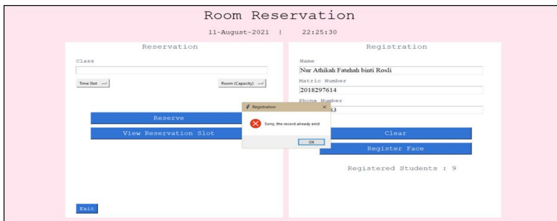
Figure 10: User existed
