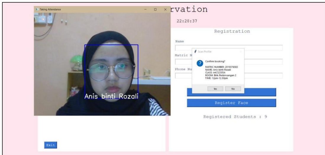
Figure 11: Reservation process
