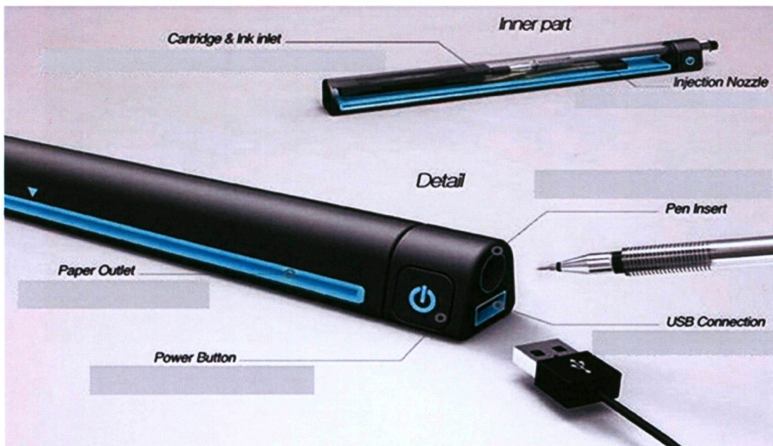
Figure 1: Pen Printer Design
