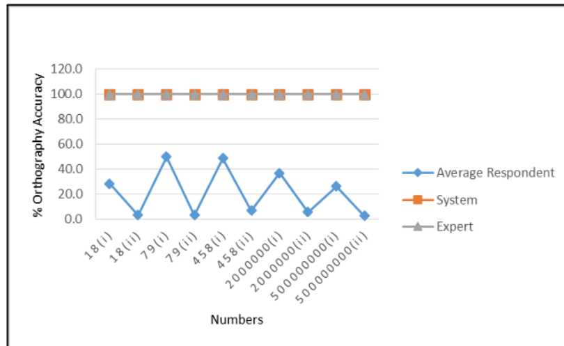
Figure 15. Orthography Accuracy
