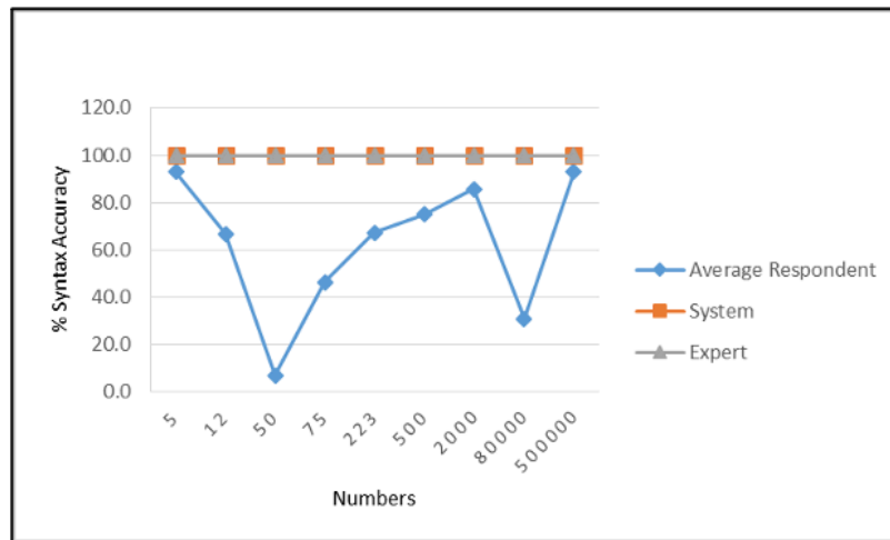
Figure 13. Syntax Accuracy
