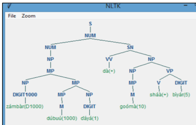
Figure 3. Parse tree for 1,000,015
