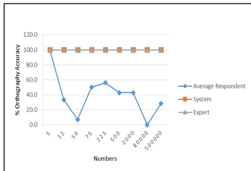
Figure 12. Orthography Accuracy
