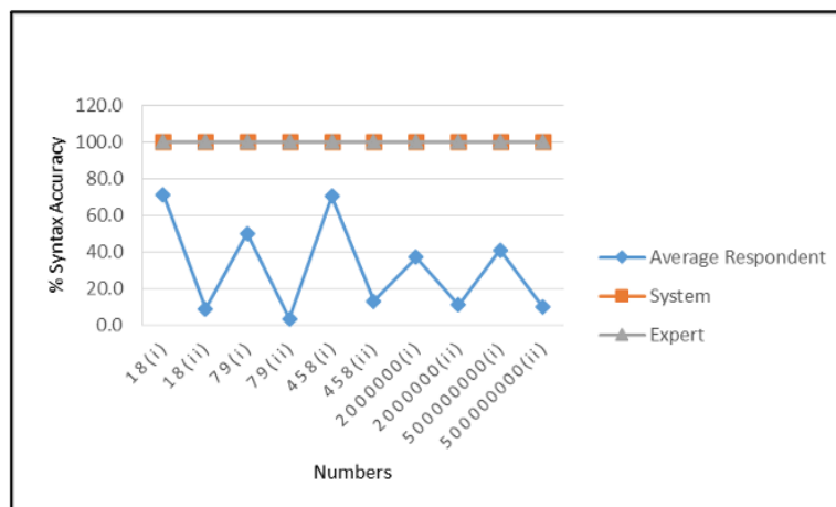
Figure 16. Syntax Accuracy
