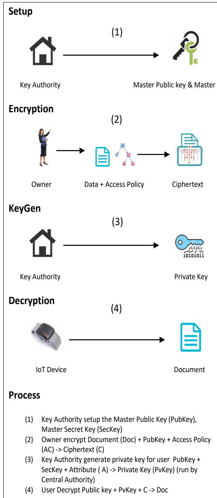
Figure 4: Four Algorithm in CP-ABE cryptography scheme
