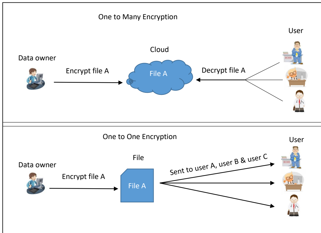
Figure 2. One to many Encryption and One to One Encryption
