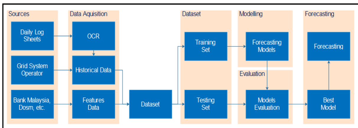
Figure 2: Modeling Framework
