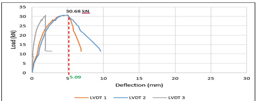
Figure 7: Load Versus Deflection Graph of the 2-Ribbed Slab (source by author)
