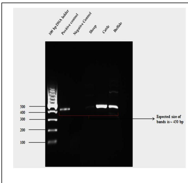
Figure 3 DNA amplification result using TOYOBO KOD FX Neo from crude sample.
