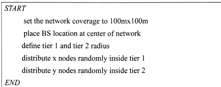
Figure 1: Algorithm 1-Initialization Phase
