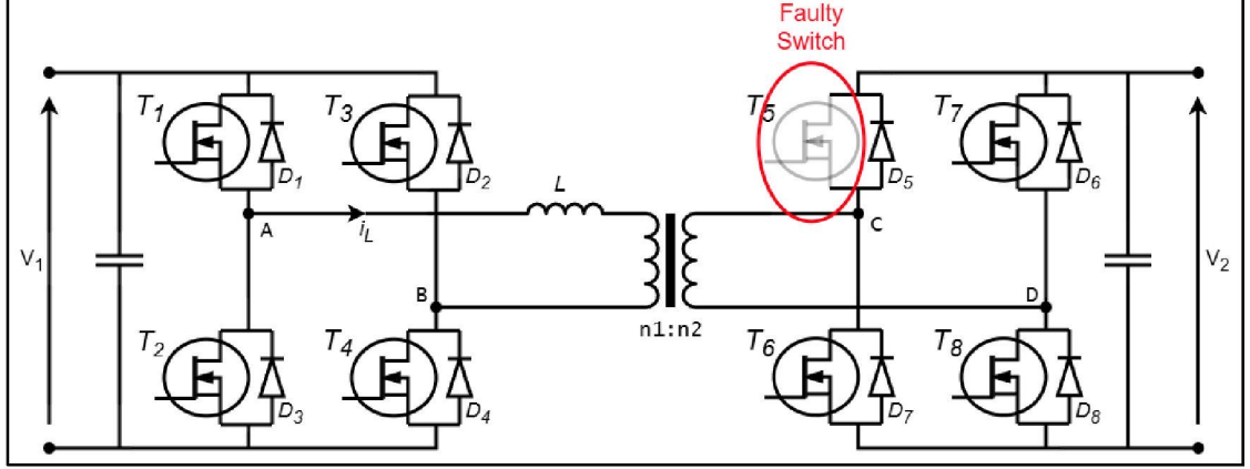
Figure 3.13 Faulty switch at T^5 for typical DAB converter
