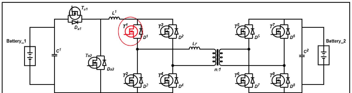
Figure 4.14 Faulty switch at T^1 for purposed DAB converter.
