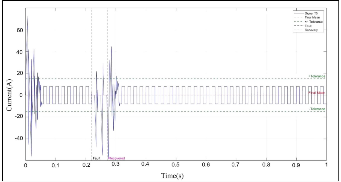
Figure 4.33 Current Waveform with Fault Detection and Stable Recovery Indication for Signal T^5
