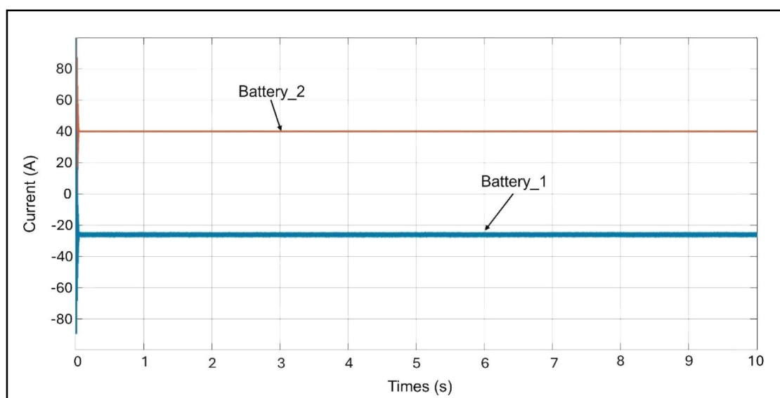
Figure 4.6 Mode 2 – Current of Battery_1 and Battery_2 vs Times.
