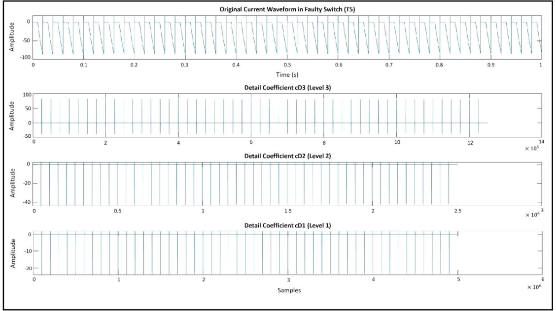
Figure 4.12 Wavelet decomposition of faulty switch ( T^5 ): Original waveform and detail coefficients (Level 1-3).
