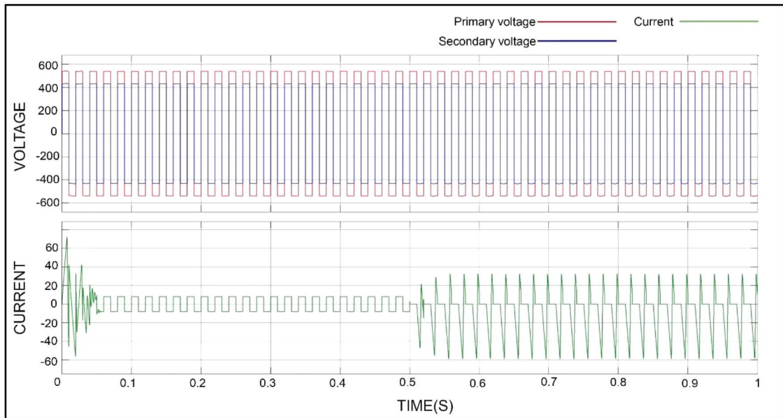
Figure 4.15 Voltage and current waveform of the DAB converter under normal and faulty condition at T^1 .
