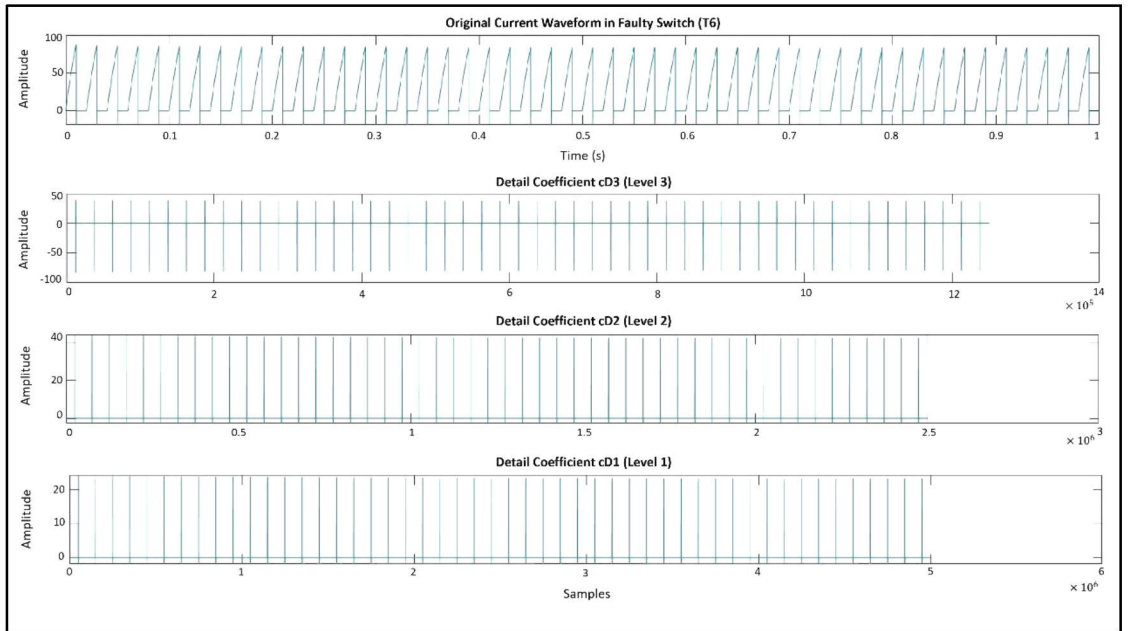
Figure 4.13 Wavelet decomposition of faulty switch ( T^6 ): Original waveform and detail coefficients (Level 1-3).
