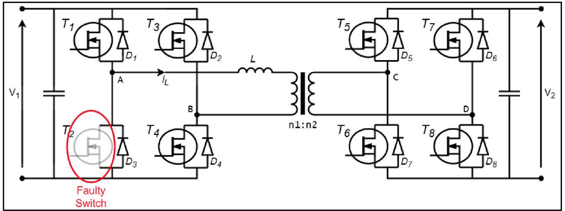
Figure 3.11 Faulty switch at T^2 for typical DAB converter.
