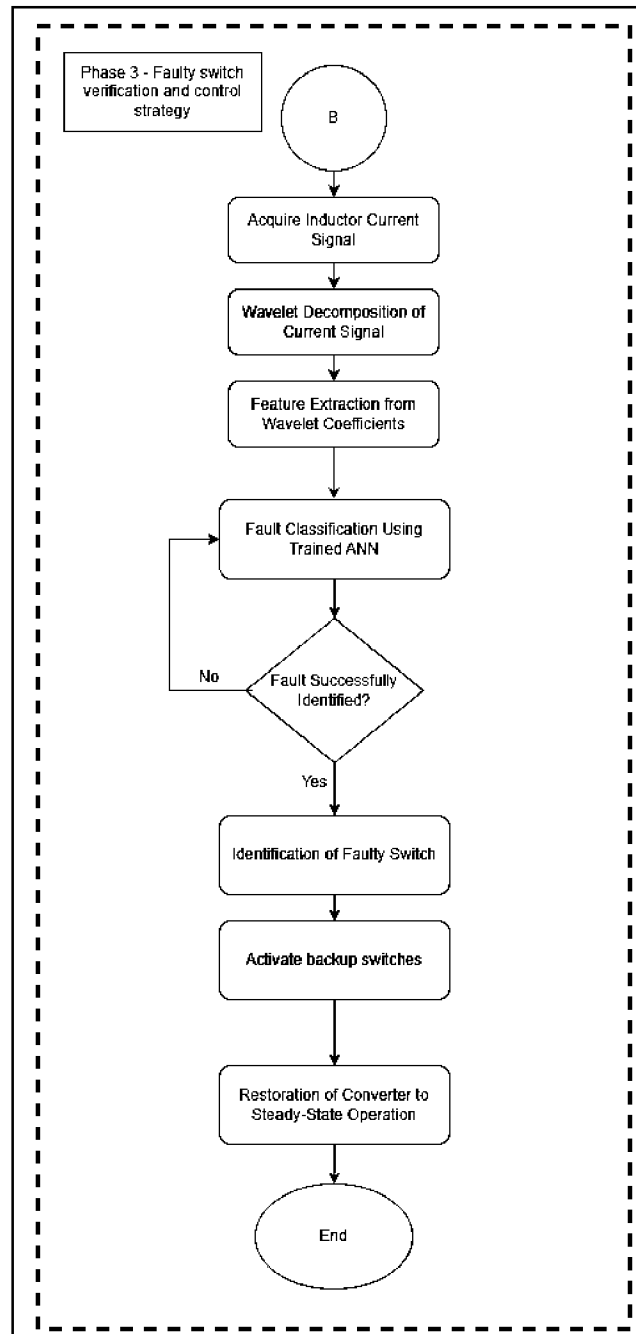
Figure 3.3 Flowchart for Phase 3
