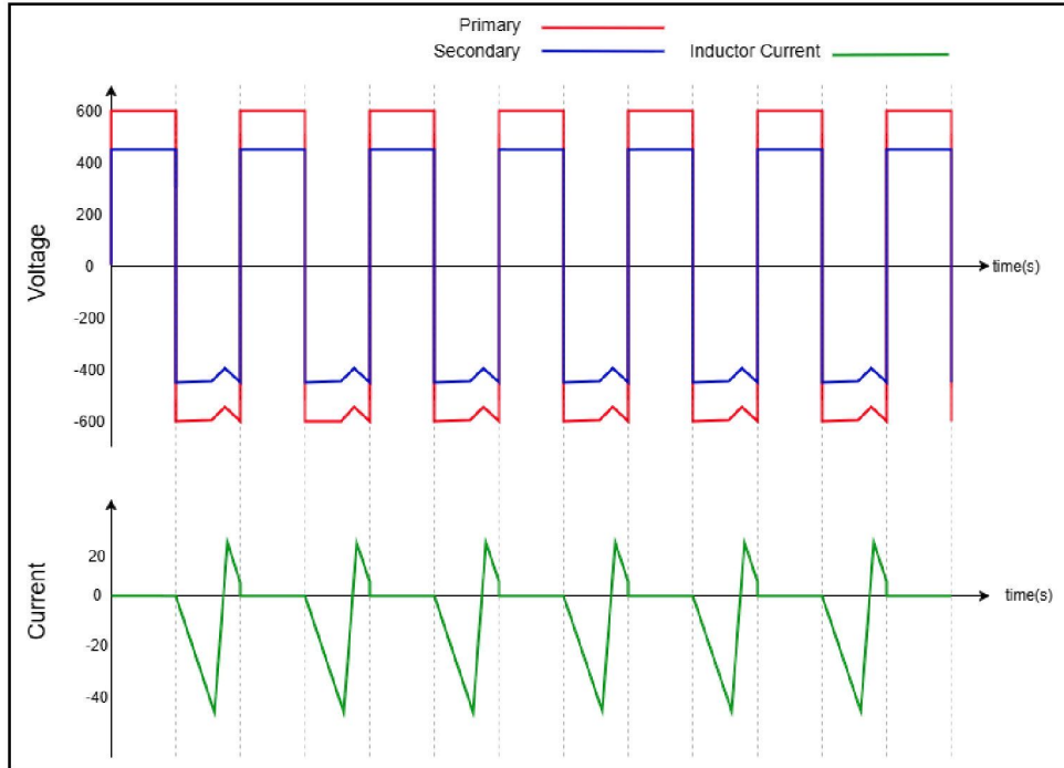
Figure 3.10 Voltage and current waveforms of DAB converter with faulty switch T^1
