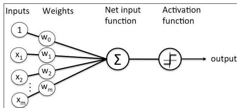
Figure 2.9 A Perceptron [77]
