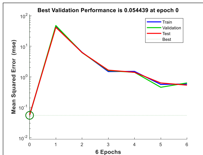
Figure 4.20 Best Validation Performance of the ANN Model for the Big Slot Size, Showing Mean Squared Error (MSE) Versus Epochs. The Lowest Validation MSE of 0.0544 Was Observed During the Early Stage of Training, After Which No Further Improvement Was Achieved
