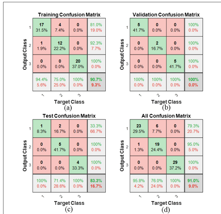
Figure 4.28 Confusion Matrices for L-band Slot Size Classification Using the SCG Algorithm: (a) Training, (b) Validation, (c) Testing, (d) Overall
