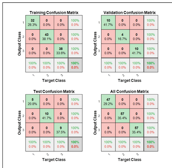
Figure 4.35 Confusion Matrices for S-band Slot Size Classification Using the SCG Algorithm: (a) Training, (b) Validation, (c) Testing, (d) Overall
