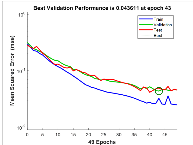
Figure 4.36 Training, Validation, and Testing Mean Squared Error (MSE) Versus Epochs For the SCG-based ANN Classifier (S-band)
