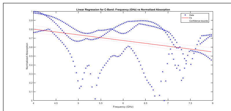
Figure 4.7 Linear Regression Analysis of Normalized Absorption within the C-Band Frequency Range
