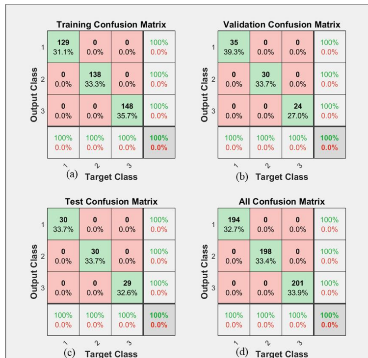
Figure 4.45 Confusion Matrices for X-band Slot Size Classification Using the LM Algorithm: (a) Training, (b) Validation, (c) Testing, (d) Overall
