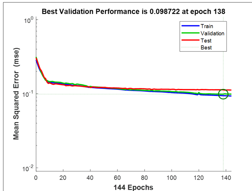
Figure 4.43 Training, Validation, and Testing Mean Squared Error (MSE) Versus Epochs For the SCG-based ANN Classifier (C-band)
