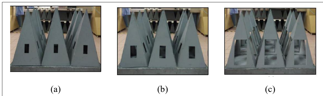
Figure 2.1 Design of Single Slot Configurations on a Biomass Hollow Pyramidal Microwave Absorbers: (a) Small Slot (b) Medium Slot (c) Big Slot [22]
