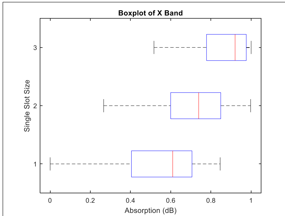
Figure 4.4 Distribution of Post-Processed X-Band Absorption Performance Data for Different Slot Sizes
