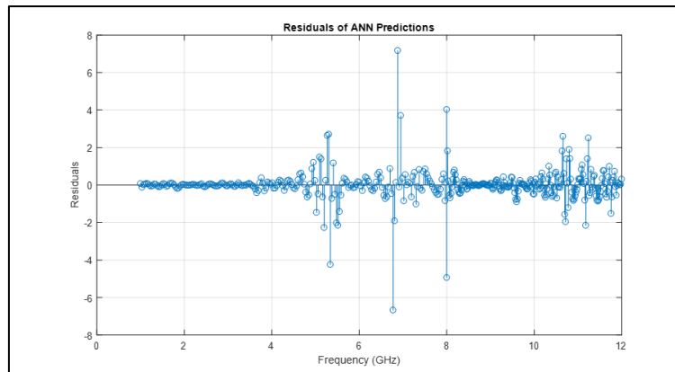
Figure 4.13 Residual Plot of ANN Model Predictions for Small Slot Size.
