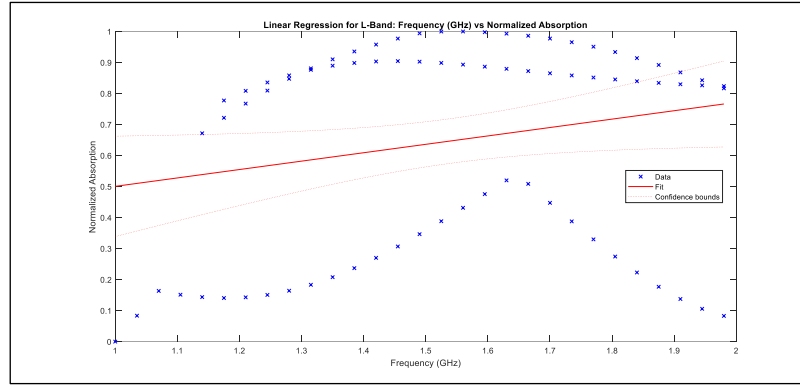
Figure 4.5 Linear Regression Analysis of Normalized Absorption within the L-Band Frequency Range
