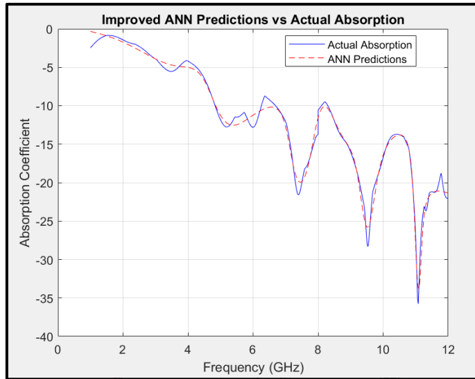
Figure 4.17 Comparison of ANN-Predicted and Actual Absorption Performance for Medium Slot Size
