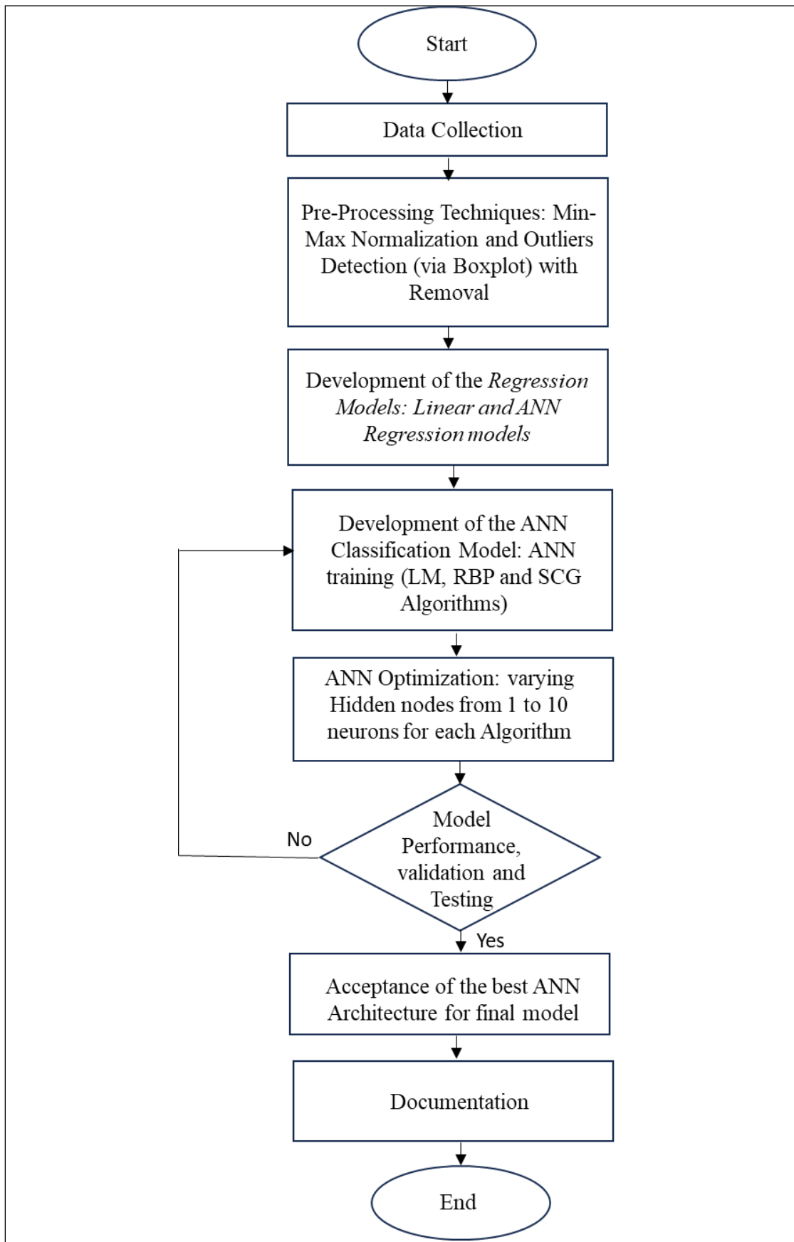
Figure 3.1 General Methodology of the Research
