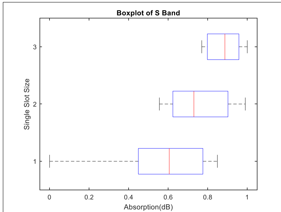
Figure 4.2 Distribution of Post-Processed S-Band Absorption Performance Data for Different Slot Sizes
