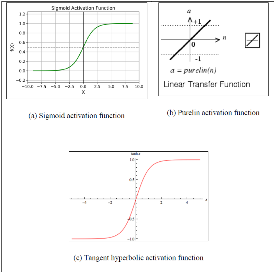
Figure 2.10 Type of Activation Functions: (a) Sigmoid Activation Function, (b) Purelin Activation Function, (c) Tangent Hyperbolic Activation Function [100], [101]
