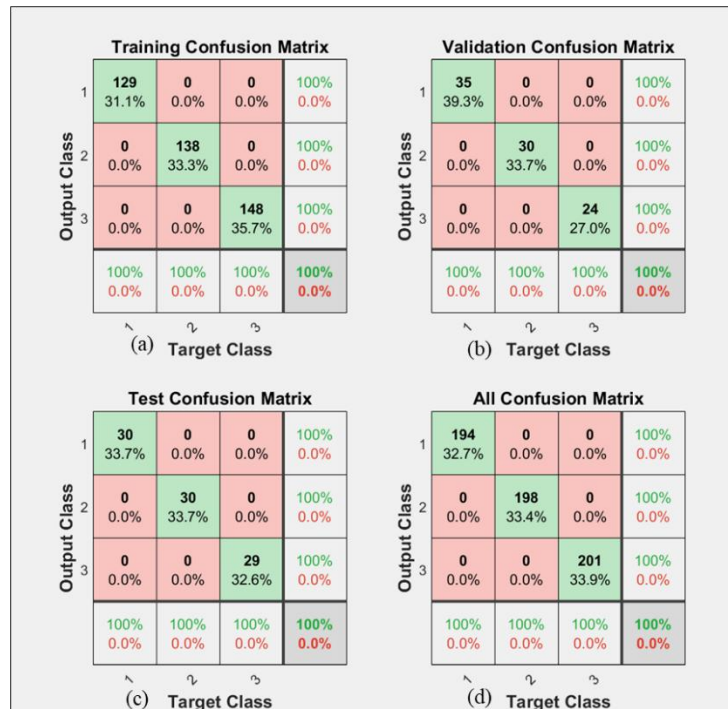
Figure 4.47 Confusion Matrices For X-band Slot Size Classification Using the RBP Algorithm: (a) Training, (b) Validation, (c) Testing, (d) Overall
