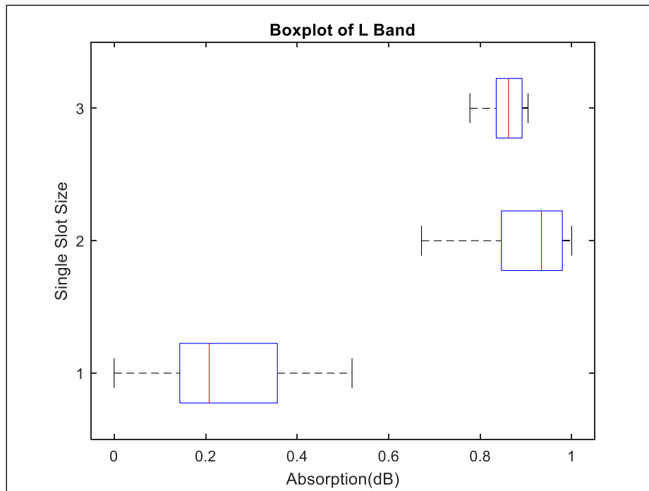
Figure 4.1 Distribution of Post-Processed L-Band Absorption Performance Data for Different Slot Sizes
