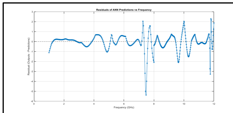
Figure 4.23 Residual Plot of ANN Model Predictions for Big Slot Size
