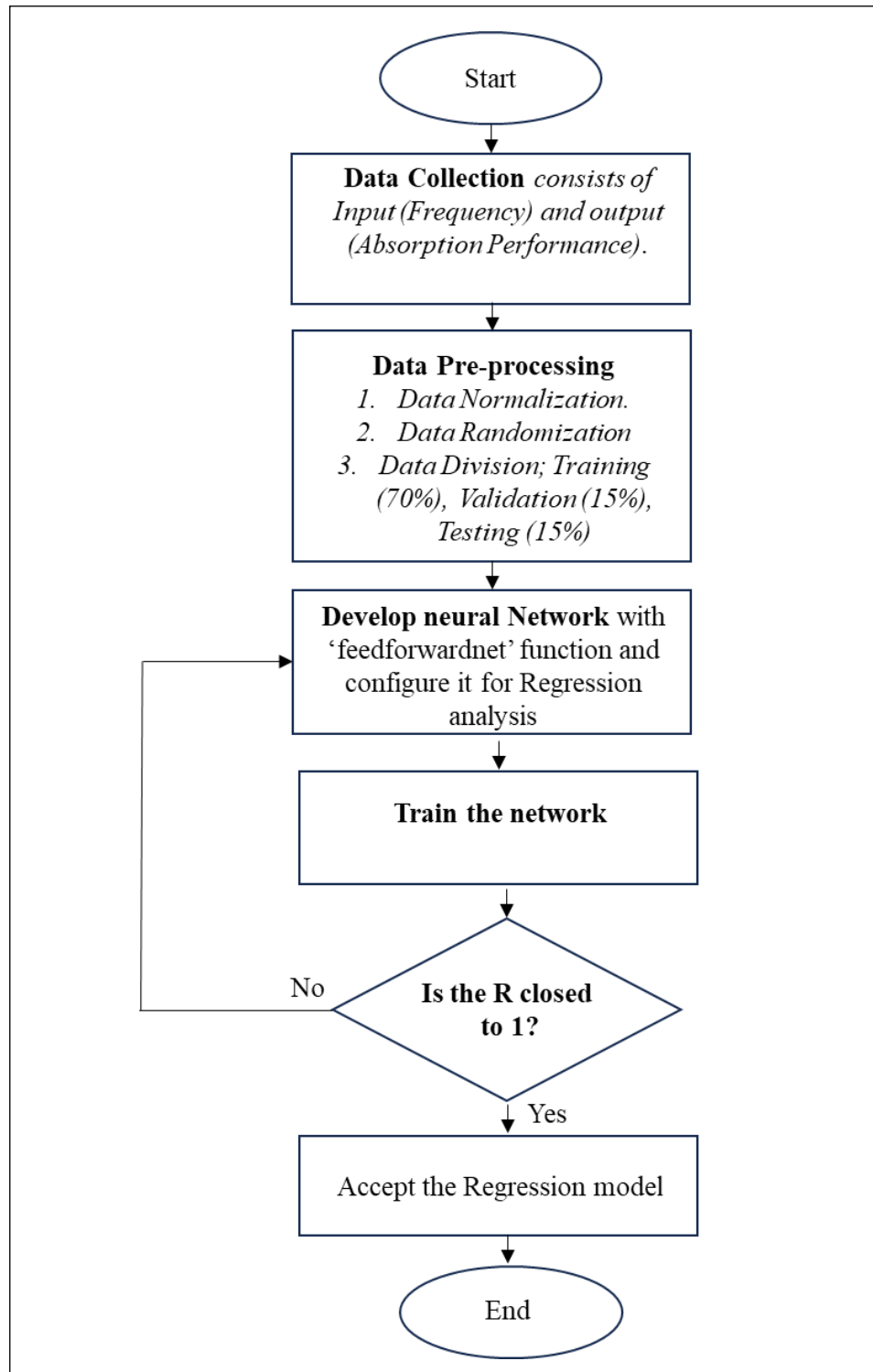
Figure 3.6 Detailed Experiment Procedure for the ANN Regression Model
