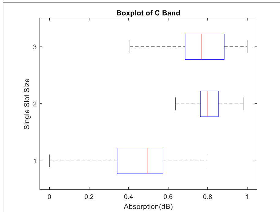
Figure 4.3 Distribution of Post-Processed C-Band Absorption Performance Data for Different Slot Sizes
