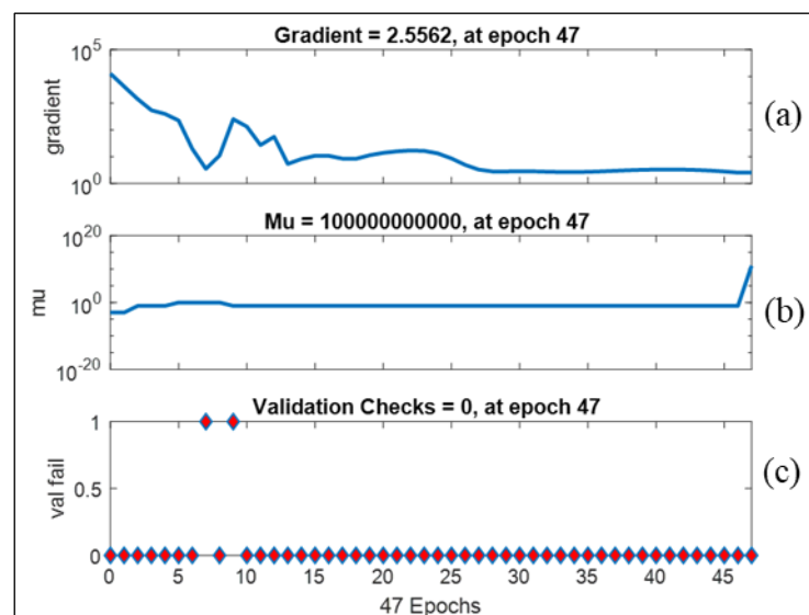
Figure 4.9 ANN Training Convergence Characteristics for the Selected Model: (a) Gradient Variation with epochs; (b) Adaptive Learning Parameter ( \mu ) Versus epochs, and (c) Validation Checks Indicating Best Validation Performance at epoch 47
