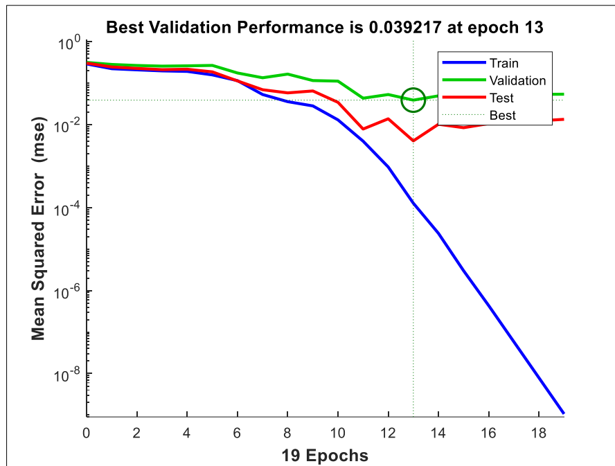
Figure 4.32 Training, validation, and Testing Mean Squared Error (MSE) Versus Epochs For the LM-based ANN Classifier (S-band)
