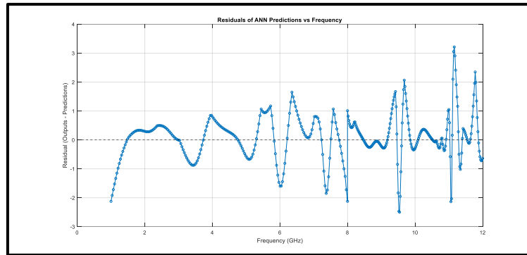
Figure 4.18 Residual Plot of ANN Model Predictions for Medium Slot Size
