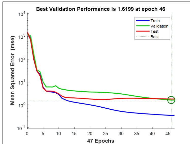
Figure 4.10 Best Validation Performance of the ANN Model showing Mean Squared Error (MSE) Versus epochs For the Training, Validation, and Testing Datasets. The Minimum Validation MSE of 1.6199 Was Achieved at epoch 46, while the Training Process Terminated After 47 epochs
