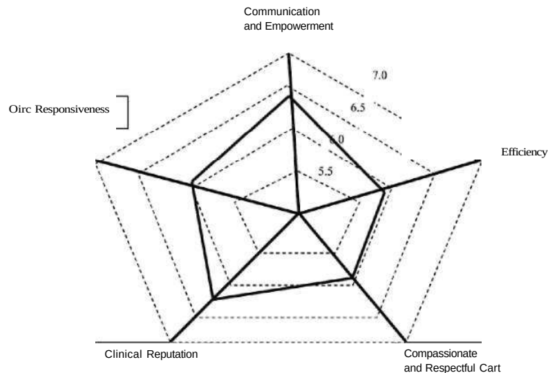
Figure 5.34 Spider-web Diagram Based on The Unweighted Scores
