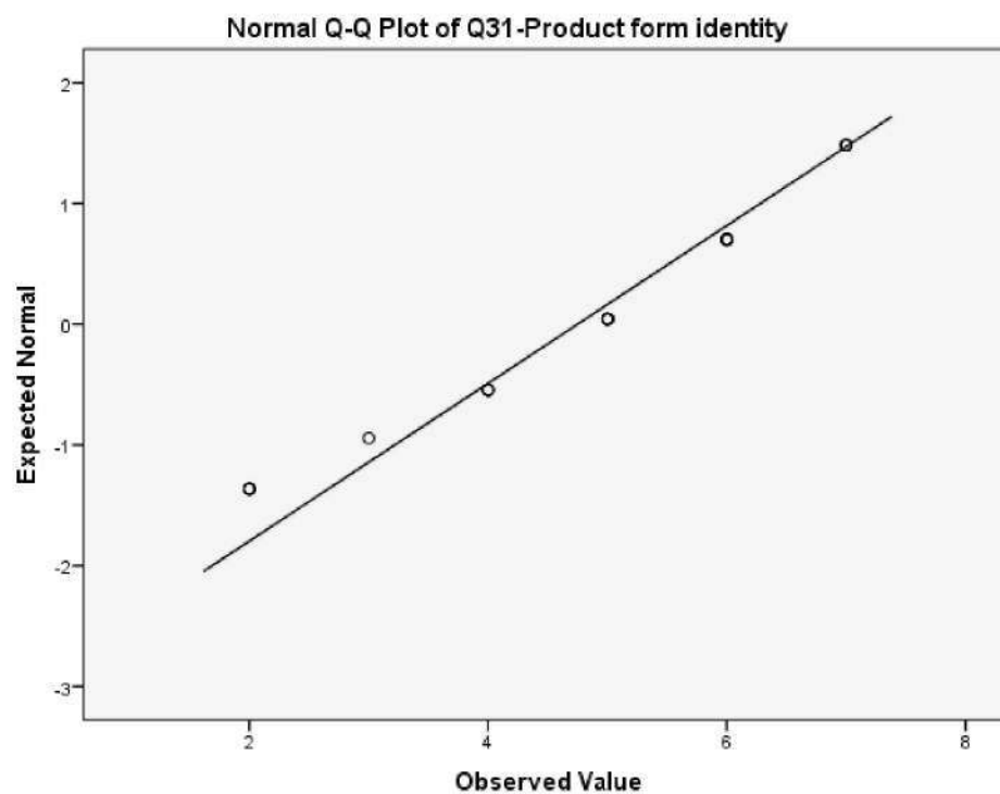
Figure 5.50 Normal Q-Q Plot SPSS for Scenario 2 - Agree
