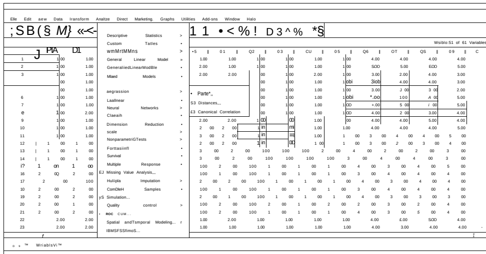
Figure 5.55 Spearman Rho SPSS for section 2: Click Analyze > Correlate > Bivariate
