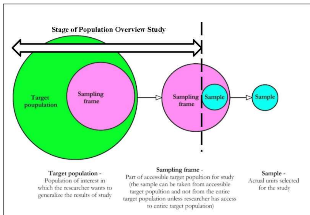
Figure 3.35 Sampling Process; Stage of Population Overview Study
