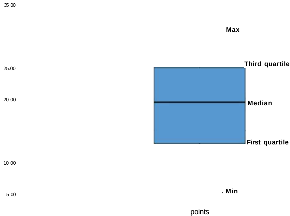
Figure 5.37 How to Interpret: A Single Box Plot in SPSS
