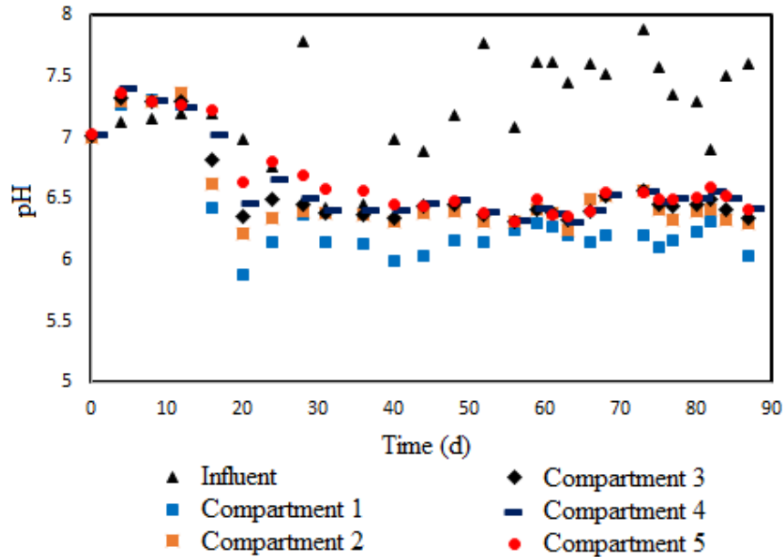
Figure 3: pH variation against various loading rates
