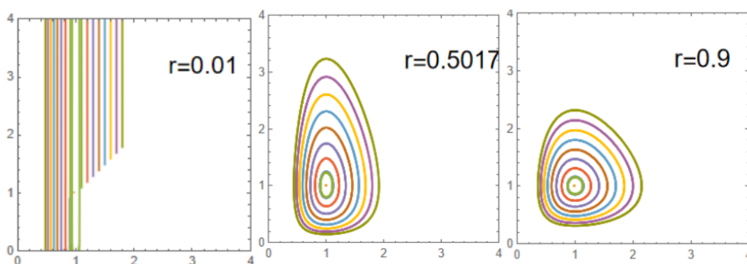
Fig. 3. Phase diagram
