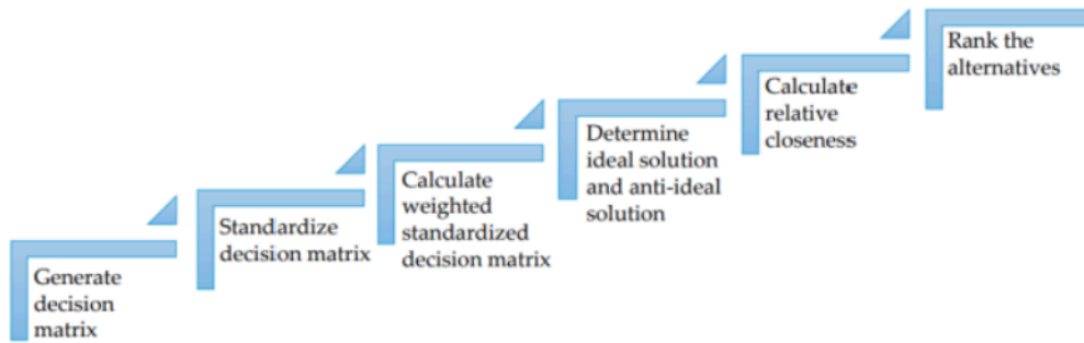
Fig. 1. Topsis process
