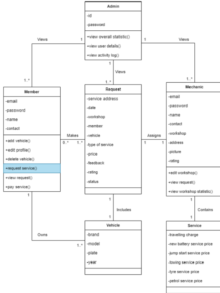
Fig. 3. Class Diagram
