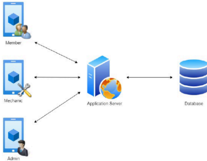
Fig. 4. Architecture Diagram
